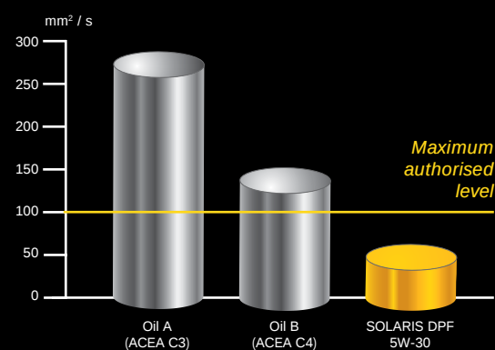
"Long Life Renault" engine test Increased viscosity at 40° C
